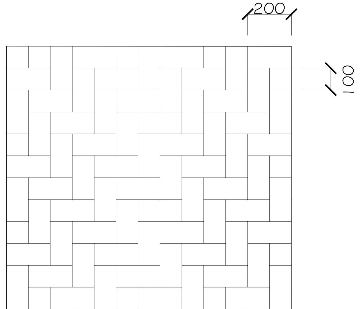
Typical Paving Pattern - Keyblok (Charcoal, 200x100x80 mm)
