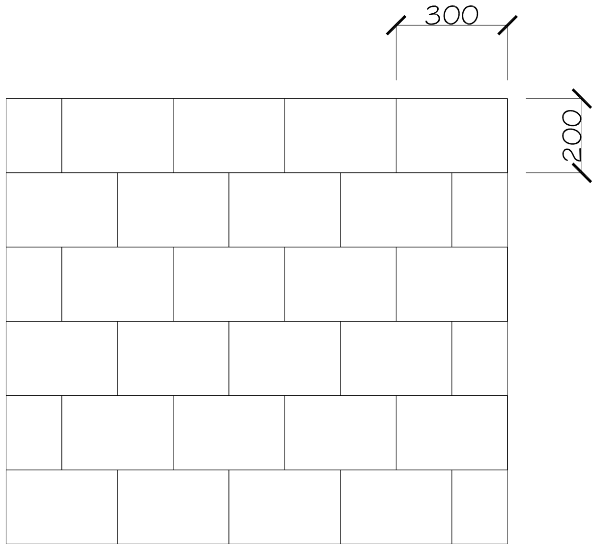
Typical Paving Pattern - Pallas (Anthracite Basalt, 300x200x80 mm)
